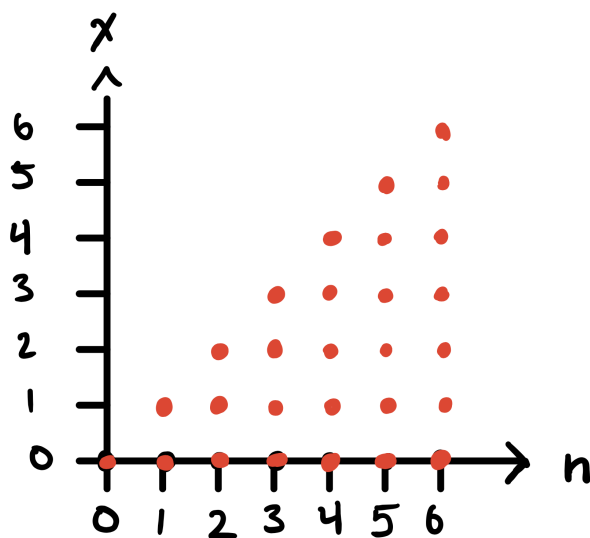
Figure 2.1: The set of pairs that (N, X) can take on in Example 2.3.
