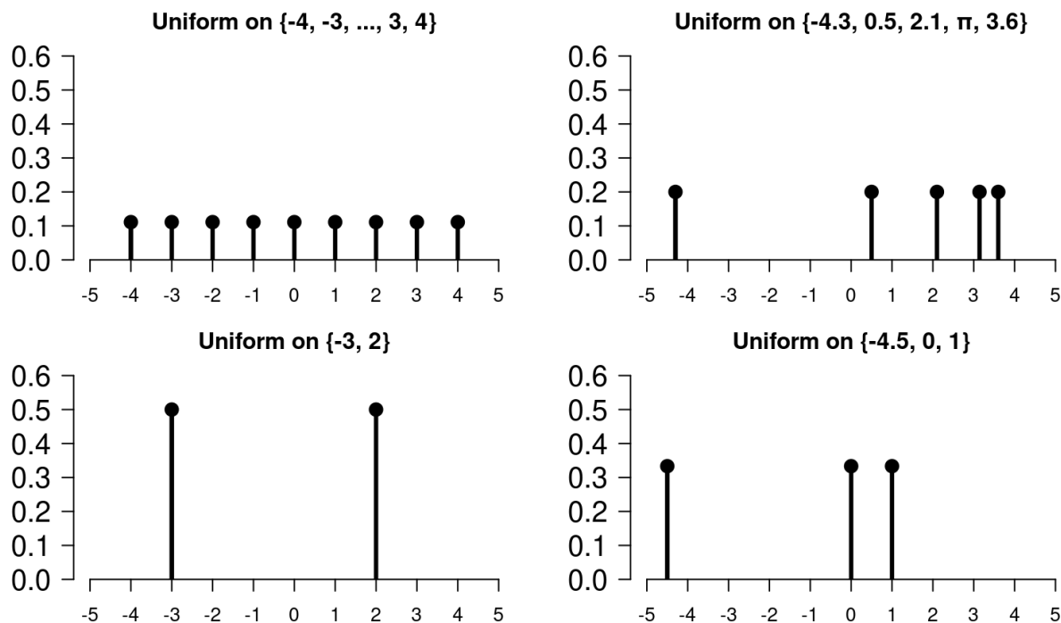
Figure 3.8: Uniform distributions on different sets of real numbers.
